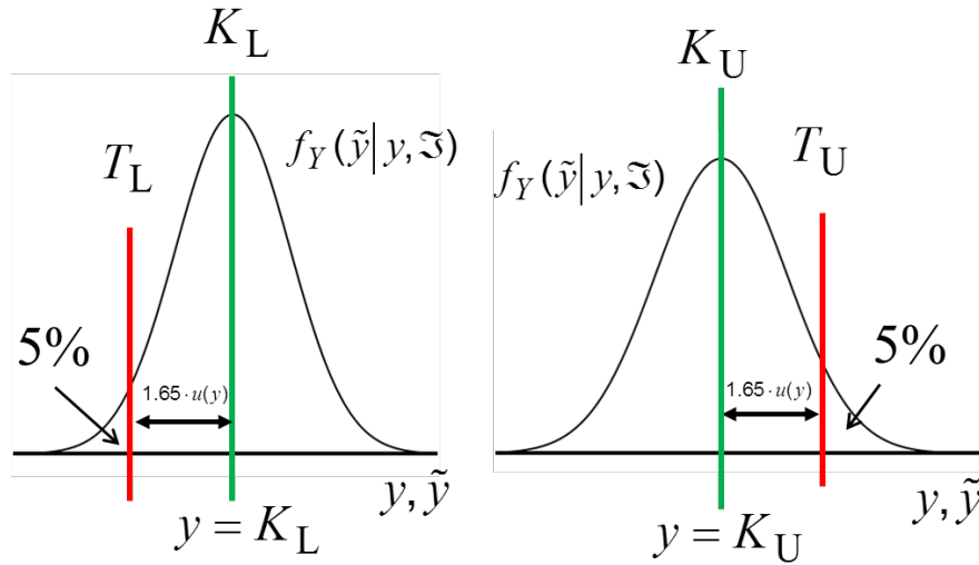
Fig. 5: Graph illustrating the acceptance interval stipulations for single upper or lower tolerance limits.
