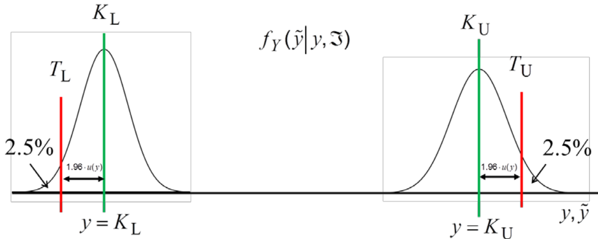
Fig. 6: Graph illustrating the acceptance interval stipulations.
