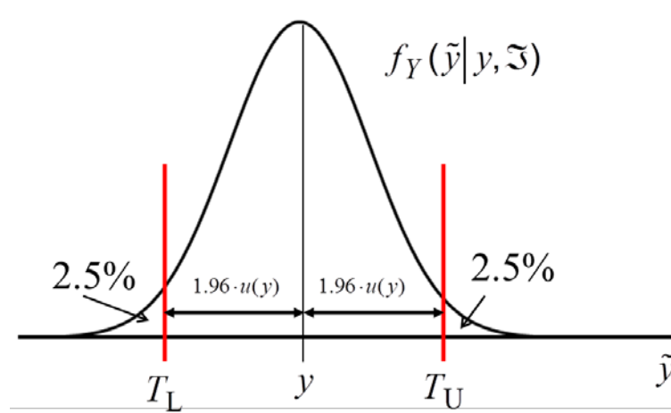
Fig. 4: Extreme case involving a two-side-limited tolerance interval that renders it necessary to apply the 95 % coverage probability for this requirement. In this extreme case, the uncertainty is so high that the probabilistically symmetric coverage interval for the 95 % probability almost fills the entire tolerance interval.
