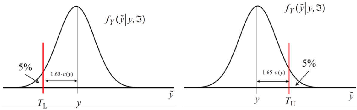
Fig. 3: Extreme cases involving single-side-limited tolerance intervals. With single-side-limited tolerance intervals, a 90 % coverage probability is sufficient for the probabilistically symmetric coverage interval in order to keep the probability of making incorrect decisions in favour of conformity at a level below 5 %.
