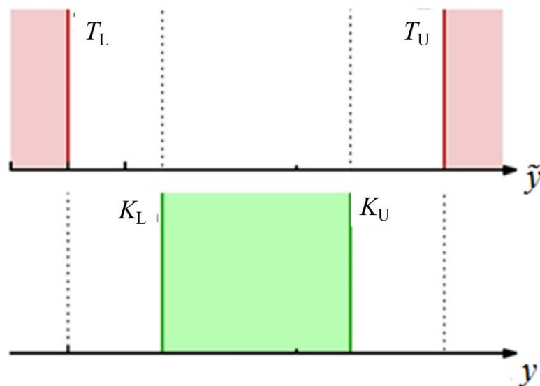
Fig. 2: Tolerance interval for the true value \tilde{y} , expressed by the bounds T_L and T_U , and acceptance interval for measured values y , expressed by K_L and K_U ; cf. also Fig. 1 in (JCGM 106).
