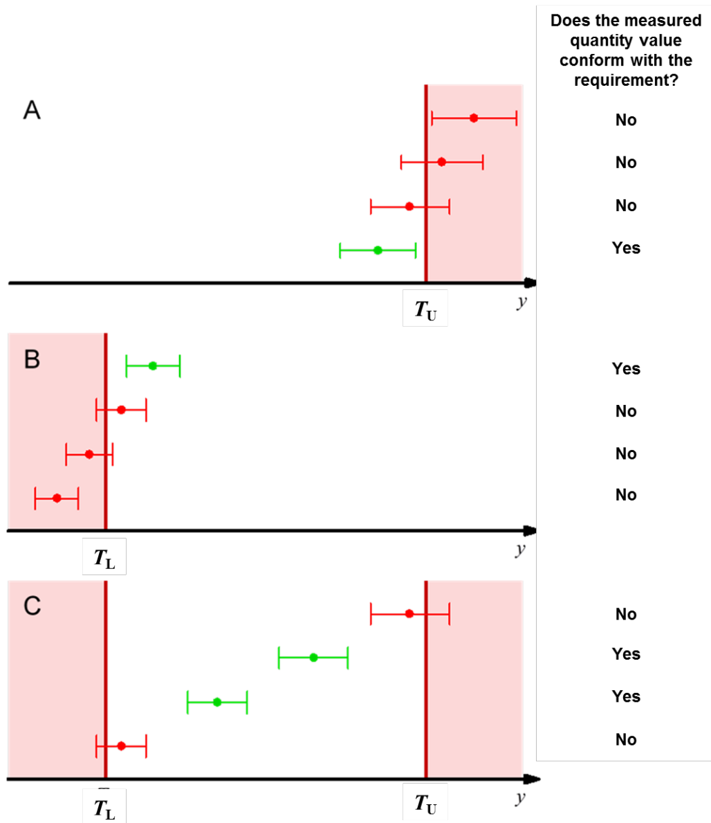
Fig. 1: Conformity test with requirements for a single-sided upwards-limited tolerance interval (A), a single-sided downwards-limited tolerance interval (B) and a two-side-limited tolerance interval (C). The SSK recommends coverage probabilities (shown above as a range of measuring points) of 90 % in cases A and B, and 95 % in case C. This recommendation is based on the criterion that the probability level for a correct decision in favour of conformity should be at least 95 %, while the probability level for an incorrect decision should not exceed 5 %.
